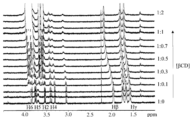
Figure 2. ^1\text{H} NMR titration of 1-adamantylmethyl \alpha -D-glucopyranoside ( 1a ) with increasing amounts of \beta -CD in \text{D}_2\text{O} at 298 K
