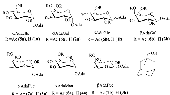
Figure 1. Molecular structure of 1-adamantylmethyl glycosides and the aglycon 1-(hydroxymethyl)adamantane
